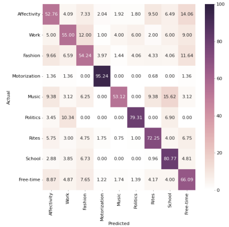
Fig. 10. Confusion matrix for the ViT-Small full-image classifier.
