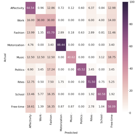
Fig. 5. Confusion matrix for the full-image classifier.
